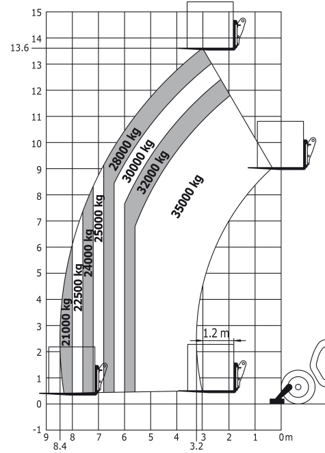
Machine on stabs with forks LC 600 mm Metric
