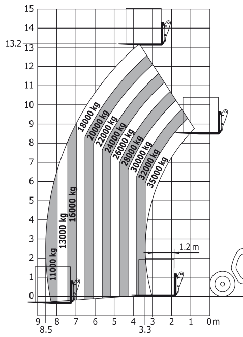
Load Chart metric
